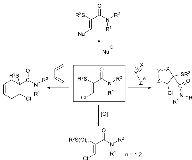
Fig. 1 Synthetic transformations of \alpha -thio- \beta -chloroacrylamides. 1–9
