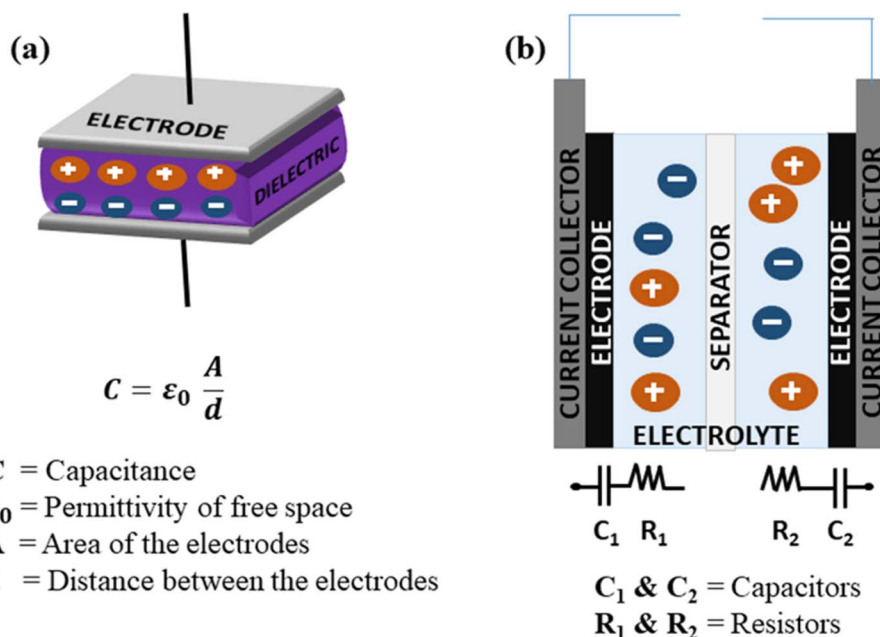
Fig. 9 Schematic of the configurations of (a) a dielectric capacitor and (b) an SC component.
