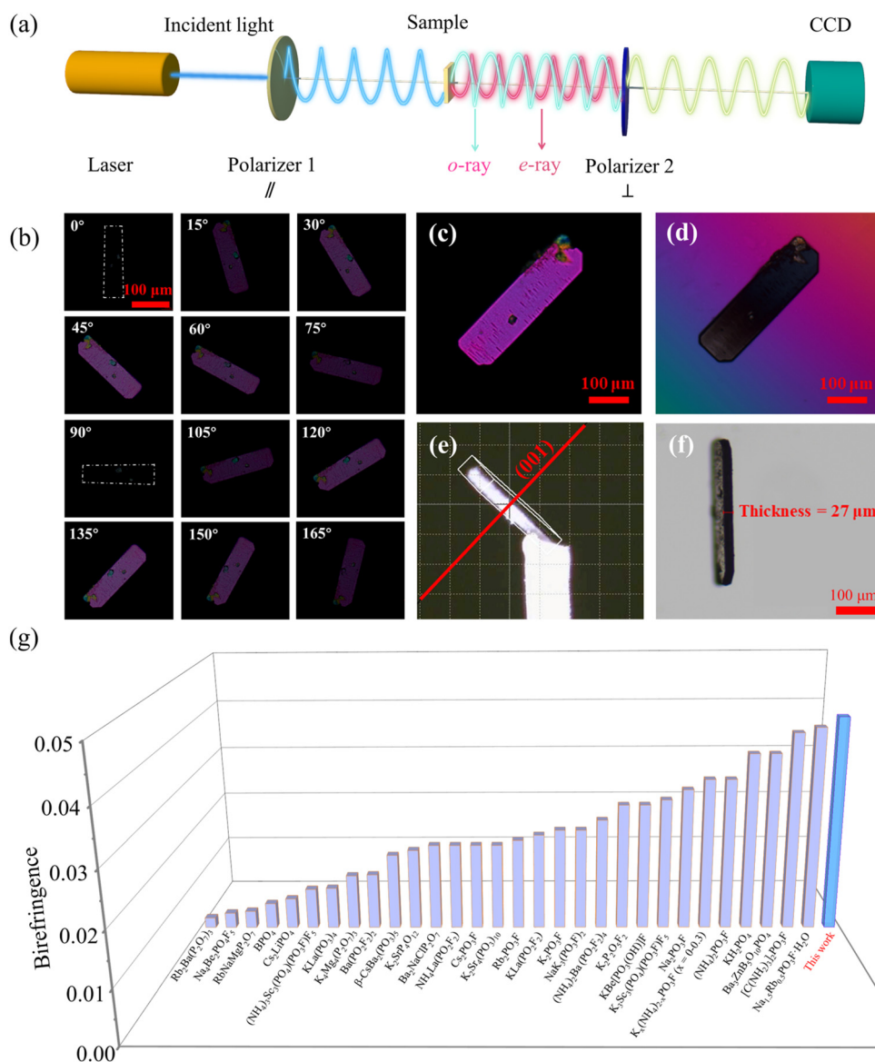
Fig. 2 Birefringence properties of KBSPF. (a) The schematic diagram illustrates the birefringence measurement using a polarizing microscope. (b) Polarized optical observations of a KBSPF crystal. The angle \varphi at which the KBSPF crystal achieves extinction is defined as 0°. (c) Original interference of the KBSPF crystal under orthogonally polarized light. (d) The corresponding crystal realizing complete extinction. (e) The orientation of the KBSPF plate used for measurement. (f) The thickness of the KBSPF crystal. (g) Comparison of the birefringence of KBSPF with many well-known phosphates and fluorophosphate optical crystals.
