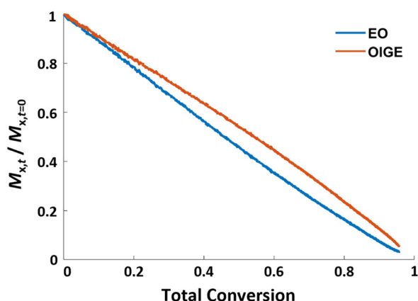
Fig. 2 Unreacted monomer versus total conversion of the in situ ^1\text{H} NMR copolymerization kinetic study of EO with OIGE. Solvent: \text{DMSO}-d_6/\text{THF}-d_8 1 : 5 (V/V), 40^\circ\text{C} .
