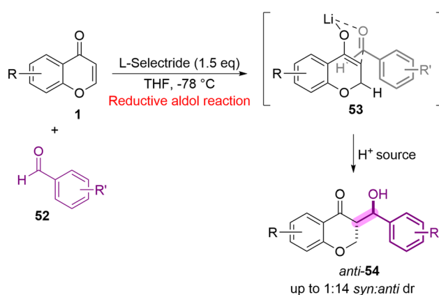
Scheme 16 Transition state 53 in the reductive aldol reaction conducted to the anti -product 54 .
