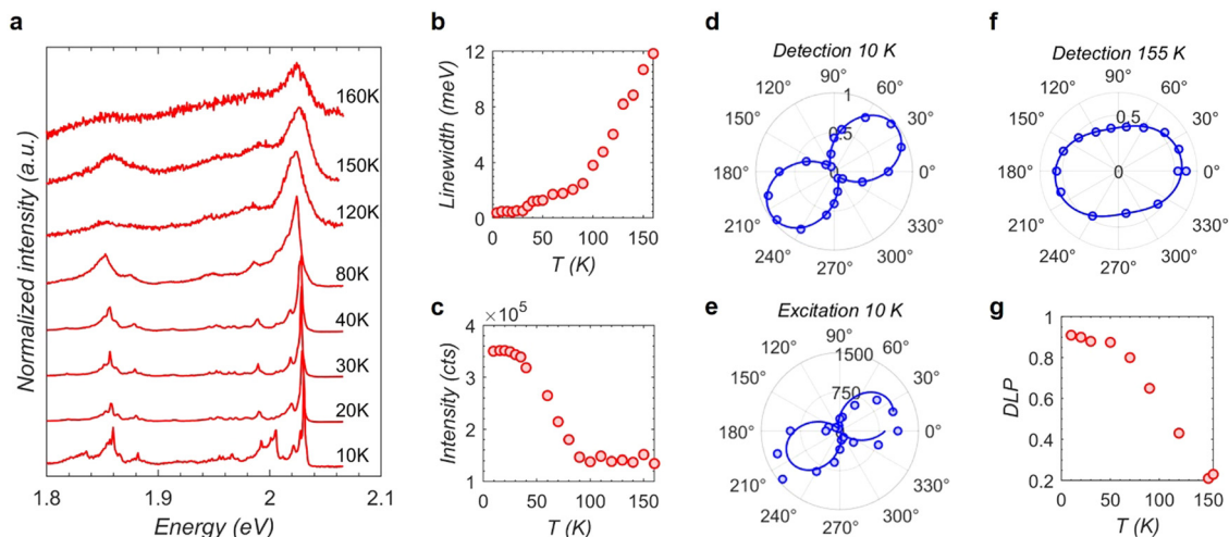
Fig. 3 Spin-correlated PL in nanoflakes. (a) Temperature-dependent PL from a nanoflake (b) and (c) linewidth and intensity display a sudden change beyond 100 K indicating a temperature-dependent PL from NFs. (d) and (e) Polar plot showing a near unity degree of linear polarization at 10 K under detection and excitation polarization analysis. (f) Polar plot showing a drop in degree of linear polarization to 20% at 155 K. (g) Degree of linear polarization for different temperatures. A residual degree of linear polarization is still present beyond the bulk T_N .
