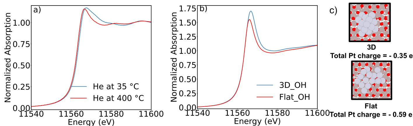
Fig. 5 Pt L_3 XANES for Pt_{1.8nm}/Al_2O_3 at 35 °C and 400 °C in (a) He. (b) Calculated Pt L_3 XANES for hemispherical and flat Pt clusters on hydroxylated Al_2O_3 . (c) Hemispherical (top) and flat (bottom) clusters on hydroxylated Al_2O_3 with total Pt charges.
