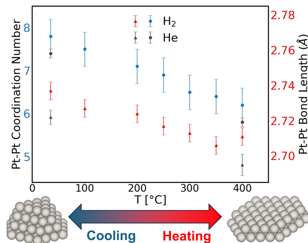
Fig. 3 Average Pt-Pt coordination number and Pt-Pt bond length (Å) under a 50% v/v \text{H}_2 and pure He between 35–400 °C. The geometrical models indicate nanoparticle shapes consistent with the coordination numbers.
