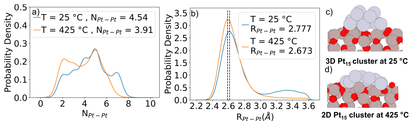
Fig. 4 Geometric statistics and trajectory snapshots of Pt_{15}/Al_2O_3 sampled via fbMC at 25\text{ °C} and 425\text{ °C} . (a, b) Predicted probability distributions for coordination number ( N_{Pt-Pt} ) and Pt-Pt bond length fit via kernel density estimation, respectively. As temperature increases, the coordination number distribution becomes broader towards lower values of N_{Pt-Pt} , suggesting that undercoordinated structures become more accessible upon heating. A decrease in average N_{Pt-Pt} is accompanied by an associated decrease in average Pt-Pt bond length. (c) Snapshot of a 3D configuration at 25\text{ °C} . (d) Snapshot of a configuration after the Pt cluster transitions to 2D at 425\text{ °C} .
