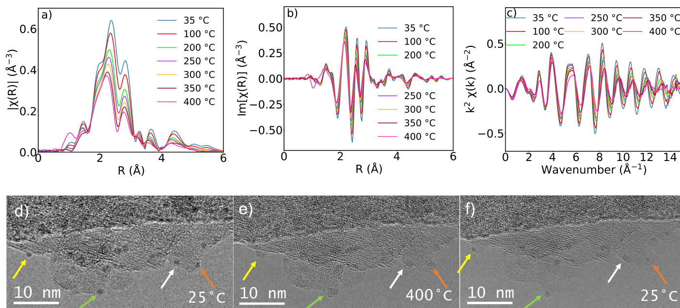
Fig. 2 Pt L_3 EXAFS spectra of Pt_{1.8\text{ nm}}/Al_2O_3 at different temperatures in 50%v/v H_2 (a) magnitude and (b) imaginary parts of the Fourier-transformed k^2 -weighted \chi(k) data in (c) ( \Delta k = 3\text{--}12\text{ \AA}^{-1} ). ETEM images of Pt_{1.8\text{ nm}}/Al_2O_3 at low (25 °C) and high (400 °C) temperatures in vacuum (d-f). The colored arrows point to the same nanoparticles at 25 and 400 °C to highlight the reversible structural changes.
