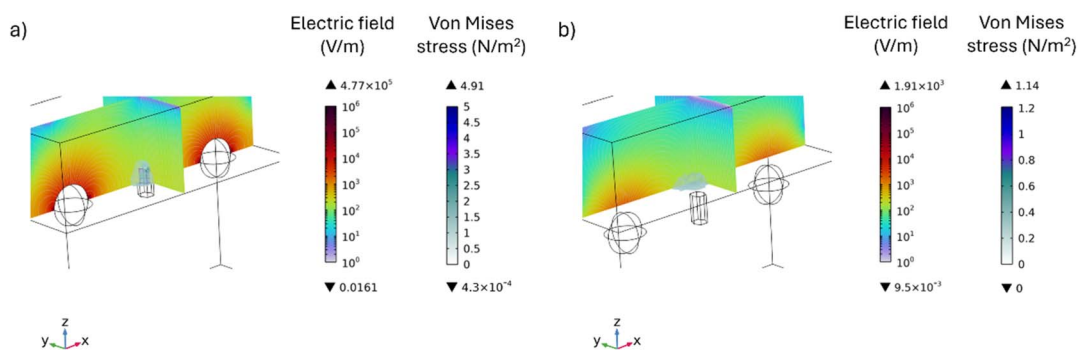
Fig. 6 Combined 3D distribution of the electric field and stress on the human cell produced by a single HAP particle placed between two MENPs under a DC field. (a) The coupled electromechanical effect for the configuration in which the HAP particle and the MENPs are at the interface between the alginate hydrogel matrix and the cell, and (b) the configuration in which the particles are fully embedded in the alginate hydrogel matrix.
