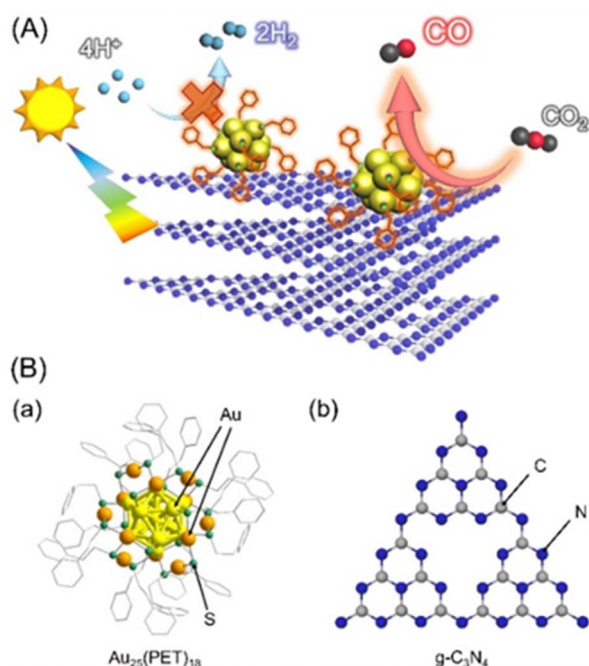
Fig. 1 (A) Schematic of the purposes of this study and (B) geometric structure of (a) \text{Au}_{25}(\text{PET})_{18} and (b) gCN photocatalysts.
