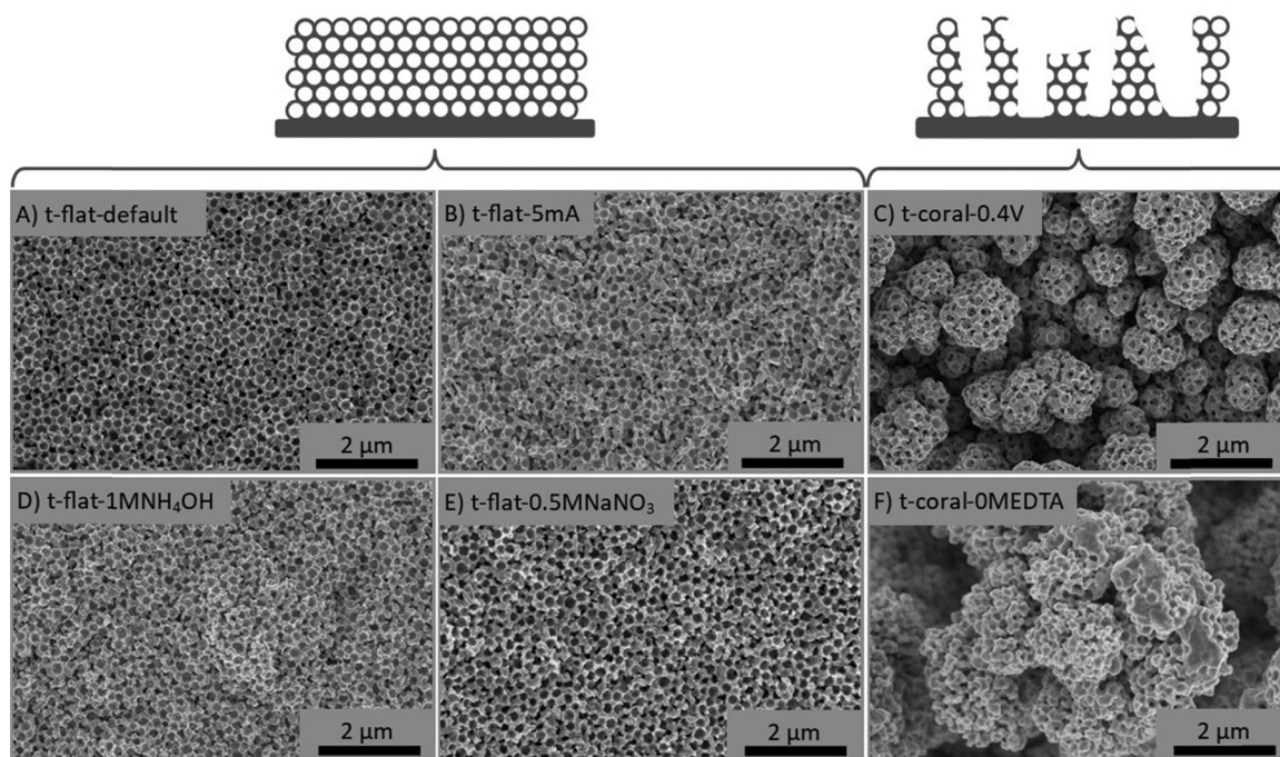
Fig. 2 SEM images of porous Ag electrodes prepared via Ag electrodeposition in voids of a PMMA sphere with different synthesis conditions: (A) default ( -0.1 V vs. Ag/AgCl, 0.05 M AgNO 3 , 1 M NaNO 3 , 0.01 M EDTA, 0.5 M NH 4 OH); (B) -5 mA; (C) -0.4 V; (D) 1 M NH 4 OH; (E) 0.5 M NaNO 3 ; (F) 0 M EDTA.
