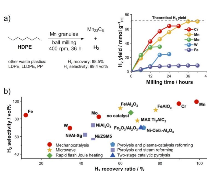
Figure 10. a) Upcycling of HDPE to high-purity hydrogen gas and metal carbide by ball milling with different metals. b) Efficiency of various methods for hydrogen generation from polyethylene. Mechanocatalysis with Mn or Cr granules provides best recoveries and selectivity. Adapted with permission from R. Gu, T. Wang, Y. Ma, T. -X. Wang, R. -Q. Yao, Y. Zhao, Z. Wen, G. -F. Han, X. -Y. Lang and Q. Jiang, Upcycling Polyethylene to High-Purity Hydrogen under Ambient Conditions via Mechanocatalysis, Angew. Chem. Int. Ed. , 2025, 64 , e202417644. 68
