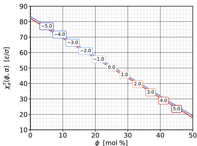
Fig. 9 Susceptibility \chi''_{\alpha|\phi} from eqn (13b) as a function of cholesterol content \phi , parametrized by different values of phospholipid abundance \alpha , as indicated in the boxed labels. The lines almost coincide, with smaller \alpha values having ever so slightly larger susceptibilities.
