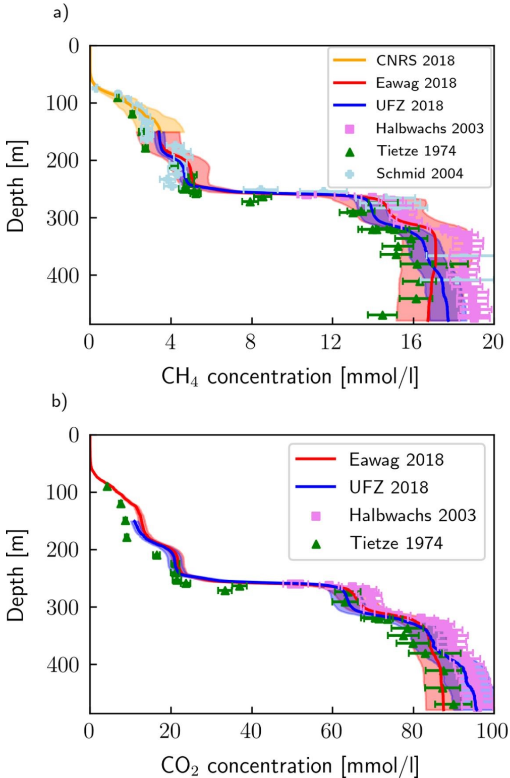
Fig. 3: Comparison between dissolved \text{CH}_4 and \text{CO}_2 concentrations measured by the 2018 campaign and those measured in 1974, 2003, and 2004. Reprinted (adapted) from reference 24. Copyright 2020 The Authors. 24
