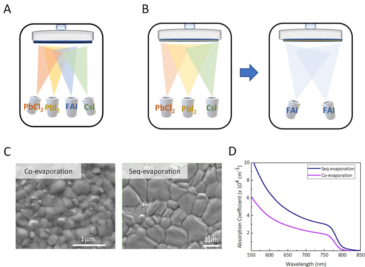
Fig. 1 (a) Schematic of co-evaporation; (b) schematic of sequential evaporation (c) SEM top micrographs of co-evaporation and sequential deposition, respectively; (d) absorption coefficient from UV-vis of films performed on sequentially evaporated and co-evaporated half stacks.
