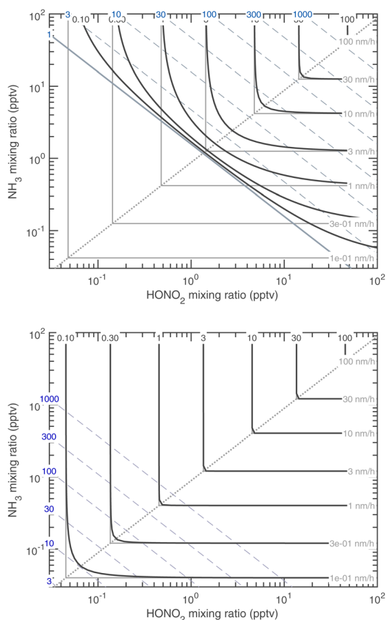
Fig. 16 Growth rate of 10 nm particles at 243 K (top) and 223 K (bottom). Note the axes shift by a factor of 100 compared to the warmer Fig. 15. At 223 K ( i.e. in the upper troposphere), the only sign of reversible (semi-volatile) condensation by the limiting reagent is curvature near the equi-collision spine with both vapors below a 1 pptv mixing ratio and almost imperceptible growth of 0.1 \text{ nm h}^{-1} .
