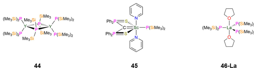
Fig. 13 Group 3 P'' complexes [Y(P'') 2 ] 2 (μ-P'') 2 ( 44 ), [Sc{C(PPh 2 ) 2 }(P'')(py) 2 ] ( 45 ), [La{P(SiMe 3 ) 2 } 3 (THF) 2 ] ( 46-La ).
