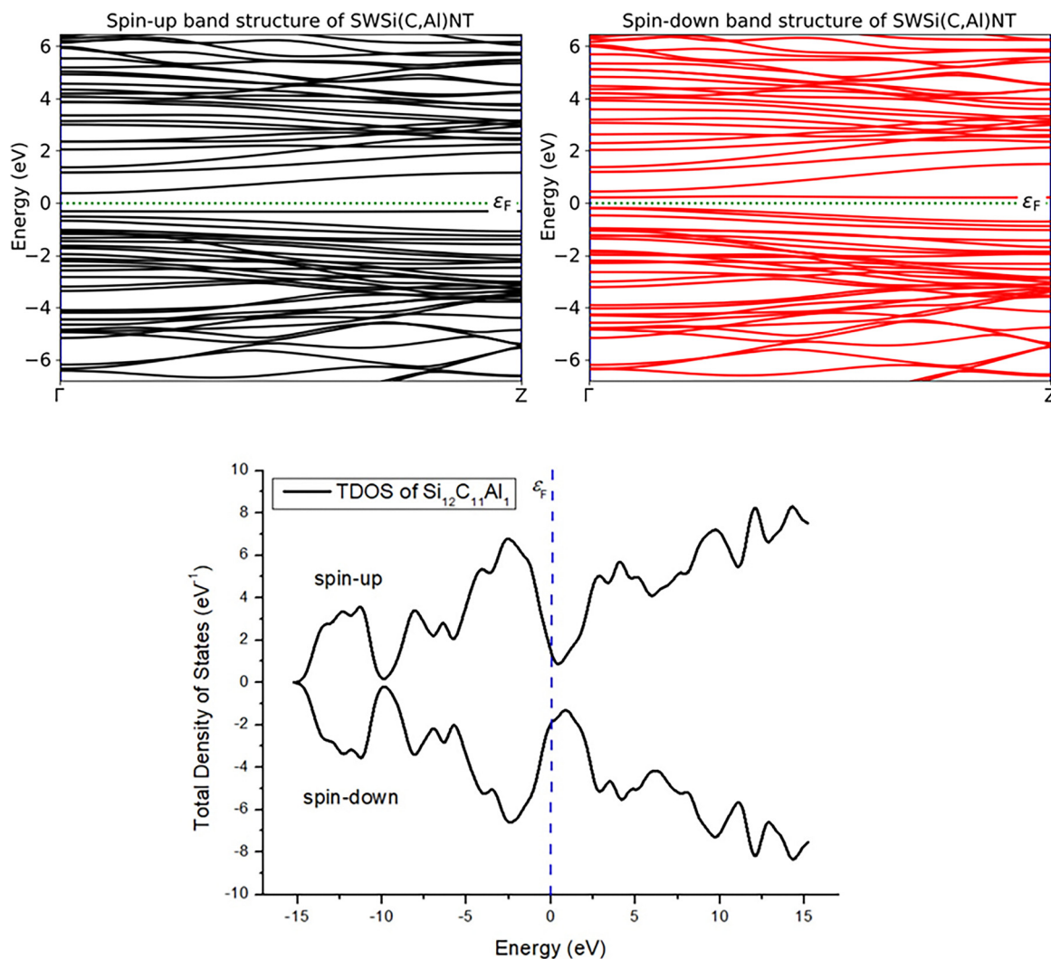
Fig. 7 Spin-up (black) and spin-down (red) band structures of \text{Si}_{12}\text{C}_{11}\text{Al}_1 NT, along with the TDOS. A spin asymmetry in the band gap is evident.
