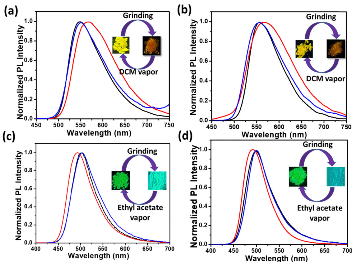
Fig. 8 Mechanochromic fluorescence spectra of (a) 2a , (b) 2b , (c) 3a and (d) 3b ( \lambda_{\text{ex}} = 370 nm), pristine sample (black curve), ground sample (red curve), and fumed with solvent vapours (blue curve). Images taken under a UV lamp at 365 nm are shown in the inset.
