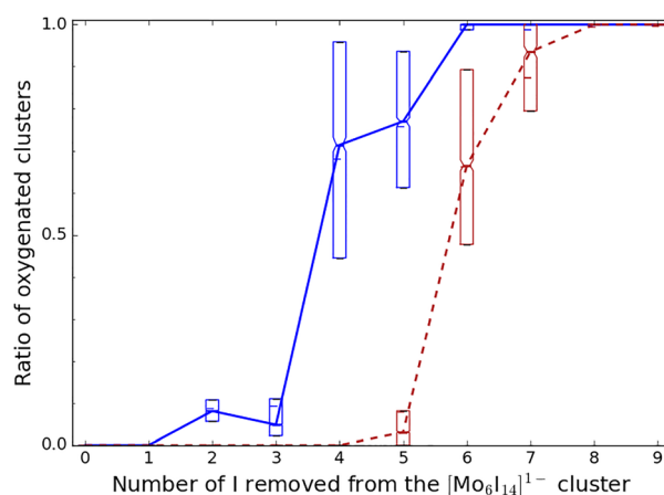
Fig. 8 Evolution, as a function of the number of I removed from the precursor, of the complex oxygenation ratio (continuous line) calculated as the sum of all (6, k, 2n)^{1-} ion intensities ( n \geq 1 ) normalized by the sum of all (6, k, 2n)^{1-} ion intensities ( n \geq 0 ). The dashed red line corresponds to the ratio of multiple oxygenation (6, k, 2n + 2)^{1-} ( n \geq 1 ) normalized by (6, k, 2n)^{1-} ( n \geq 0 ). Data are averaged from the 4 experimental fragmentation ranges in the UV and visible ranges.
