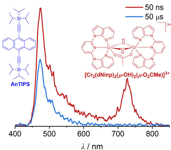
Fig. 3 Photon upconversion luminescence spectra of the Cr(III) dimer/AnTIPS pair in deaerated acetonitrile/toluene (1 : 1) at 20 °C with 50 ns (red traces) and 50 \mu\text{s} (blue traces) time delays after excitation at 532 nm (pulse energy of \sim 50 mJ), together with the molecular structures of the upconversion pair. 112 Reproduced under terms of the CC-BY license from ref. 112. Copyright 2024, Wiley-VCH.
