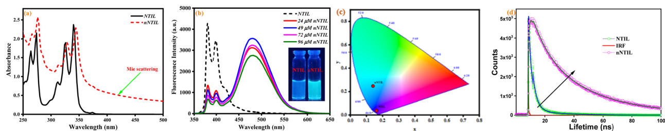
Fig. 1 (a) UV-visible absorption spectra of NTIL (49 \mu M) and nNTIL (49 \mu M). (b) Fluorescence spectra of NTIL and nNTIL in different amounts of NTIL. (c) CIE diagram of NTIL and nNTIL. (d) Photoluminescence lifetime decays of NTIL in THF and nNTIL in water.
