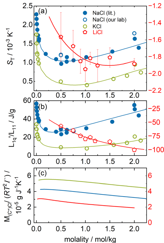
Fig. 2 (a) Soret coefficients of sodium and potassium chloride in water as a function of molality at T = 25 \text{ }^\circ\text{C} . We used the Soret coefficients of NaCl (filled blue symbols) and KCl (open green symbols) from the literature 16,32–37 and we added our TDFRS measurements (open blue symbols). For comparison, we show the recently published data for lithium chloride at T = 25 \text{ }^\circ\text{C} . 22 Note that in all three parts of the figure, the data for LiI are plotted against the right red y-axis. The red line in the case of LiCl corresponds to the green line in Fig. 5 in ref. 22, where the Onsager ratio was approximated by an exponential function. The solid lines for NaCl and KCl are a guide for the eye. (b) The ratio of the phenomenological Onsager coefficients L'_{1q}/L_{11} for NaCl and KCl at 25 \text{ }^\circ\text{C} calculated from the experimental data according to eqn (3). The solid lines are a guide to the eye. (c) M_{(C*)Cl}/(RT^2\Gamma) at 25 \text{ }^\circ\text{C} for sodium and potassium chloride. C^* stands for the corresponding cation. Further details can be found in the text.
