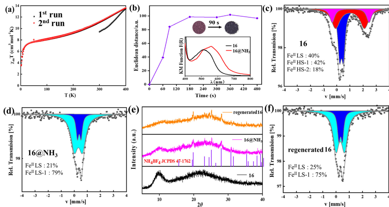
Fig. 15 (a) \chi_m T vs. T plots for microcrystalline cage 16. (b) Response time curve of 16 to \text{NH}_3(\text{g}) at room temperature. ^{57}\text{Fe} Mössbauer spectrum of 16 (c), 16@ \text{NH}_3 (d) and regenerated 16 (f). PXRD patterns of 16, 16@ \text{NH}_3 and regenerated 16 (e). 91
