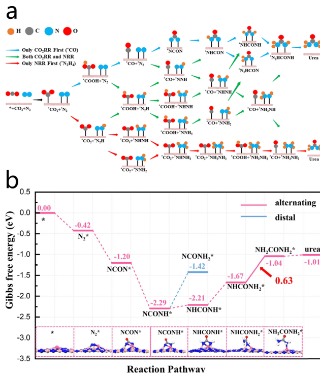
Fig. 5 (a) Mechanism diagram of the electrochemical coupling of \text{CO}_2 and \text{N}_2 to produce urea. Reproduced with permission from ref. 37. Copyright 2023, Journal of Materials Chemistry A. (b) Reaction energy barriers and the corresponding intermediate structures for urea electrosynthesis on the Fe/p-BN catalyst. Reproduced with permission from ref. 39. Copyright 2023, Chemical Engineering Journal.
