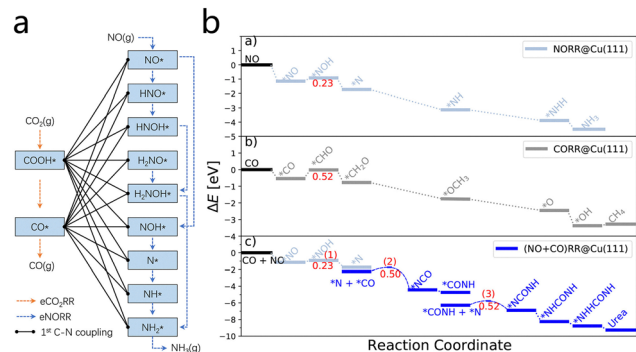
Fig. 4 (a) Schematic illustration of \text{eCO}_2\text{RR} , \text{eNORR} , and the first C–N coupling reactions. Reproduced with permission from ref. 34. Copyright 2024, ACS Catalysis. (b) Three reaction pathways on the Cu(111) surface energy diagram. Reproduced with permission from ref. 36. Copyright 2023, ACS Catalysis.
