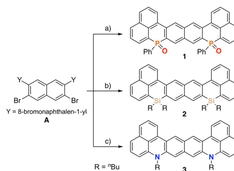
Scheme 1 Reaction conditions for the synthesis of hexaarenes 1 , 2 and 3 . Conditions: (a) 1. ^t\text{BuLi} , -80\text{ }^\circ\text{C} ; 2. \text{PhPCL}_2 ; 3. \text{H}_2\text{O}_2 . (b) 1. ^t\text{BuLi} , -80\text{ }^\circ\text{C} ; 2. ^t\text{Bu}_2\text{SiCl}_2 . (c) \text{Pd}_2(\text{dba})_3 , R -BINAP, \text{NaO}^t\text{Bu} , ^t\text{BuNH}_2 .
