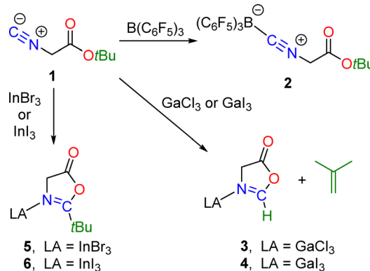
Scheme 2 Synthesis of 2–6 .
