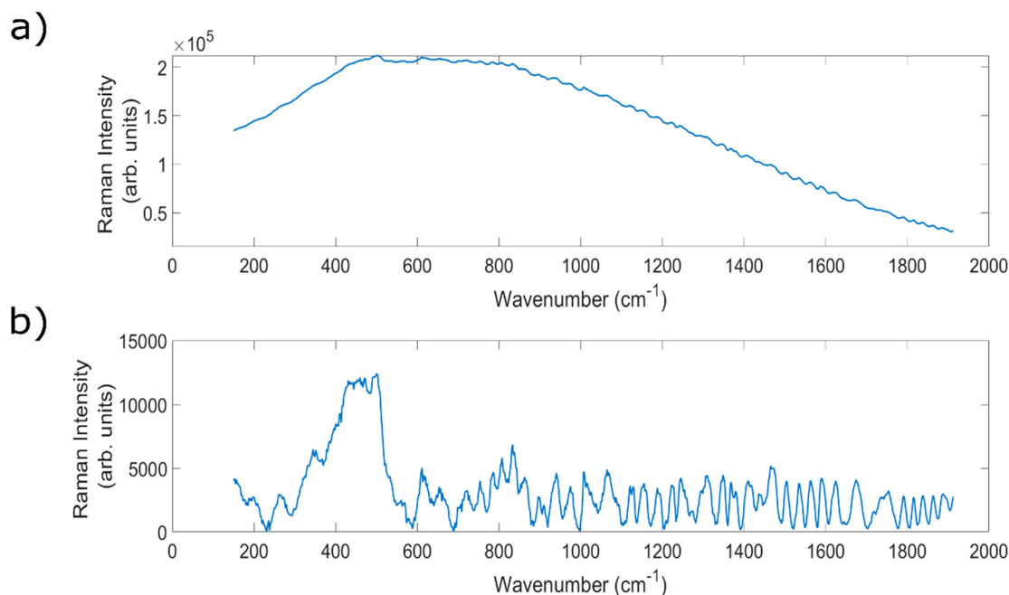
Fig. 1 (a) An example of a highly fluorescent, raw Raman spectrum of porcine liver (a particularly fluorescent organ) taken using a fibre optic Raman probe at 830 nm. Mean of 15 × 40 second spectral measurements. (b) Corresponding baselined spectrum.
