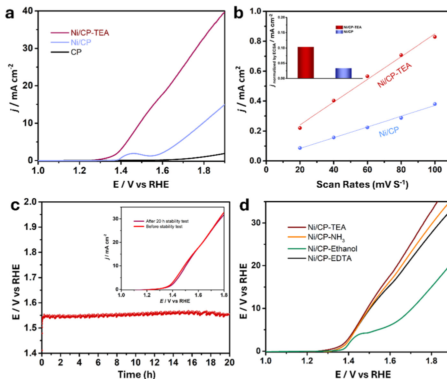
Fig. 3 (a) Linear sweep voltammetry (LSV) polarization curve of Ni/CP-TEA, Ni/CP and CP at a scan rate of 5 mV s -1 in 0.1 M KOH. (b) The ratio of current density against different scan rates based on the CV curves. Inset: Comparison of the current density normalized by the ECSA at an overpotential of 400 mV. (c) Chronopotentiometry curve of Ni/CP-TEA at 10 mA cm -2 . The inset shows the LSV polarization curves of Ni/CP-TEA before and after the stability test. (d) LSV polarization curve of Ni/CP-TEA, Ni/CP-NH 3 , Ni/CP-EDTA and Ni/CP-ethanol at 5 mV s -1 in 0.1 M KOH.
