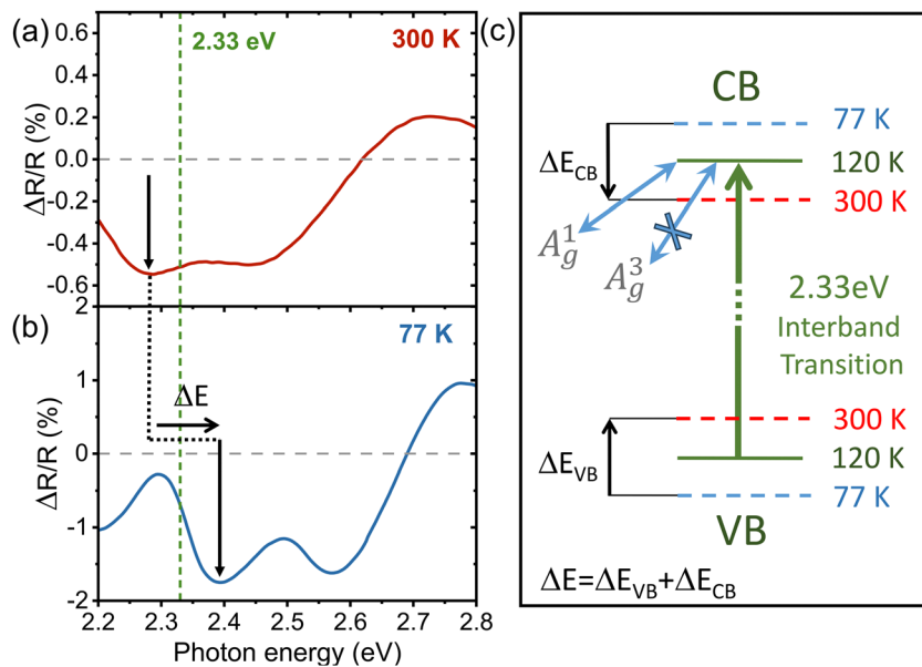
Fig. 6 Transient reflectivity measurements of \text{PdSe}_2 measured at (a) 300 K and (b) 77 K showing the differential reflectivity, \Delta R/R at 1 picosecond time delay after photoexcitation. The arrows indicate the shift of the transition around 2.33 eV toward higher energies as the sample temperature is reduced. (c) A schematic representation of the variation in some interband optical transitions, showing how resonant excitation at 120 K interacts differently with various phonon modes.
