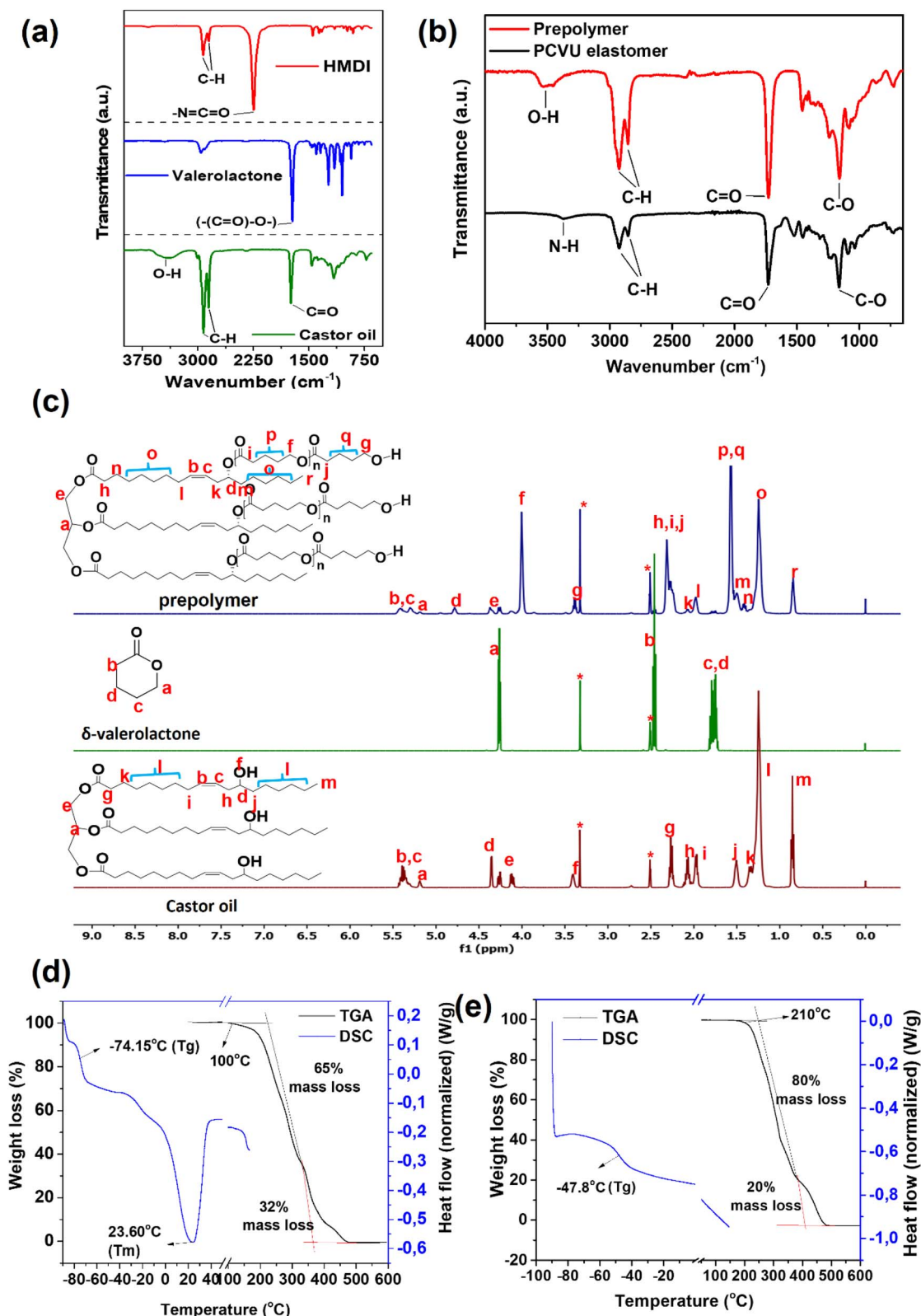
Fig. 2 (a) FT-IR profiles of starting monomers castor oil, \delta -VL, and HMDI. (b) FT-IR profiles of prepolymer and PCVU elastomer. (c) ^1\text{H} -NMR profile of prepolymer with the comparison of starting monomers castor oil and \delta -VL. (d) TGA and DSC profiles of prepolymer and (e) PCVU elastomer.
