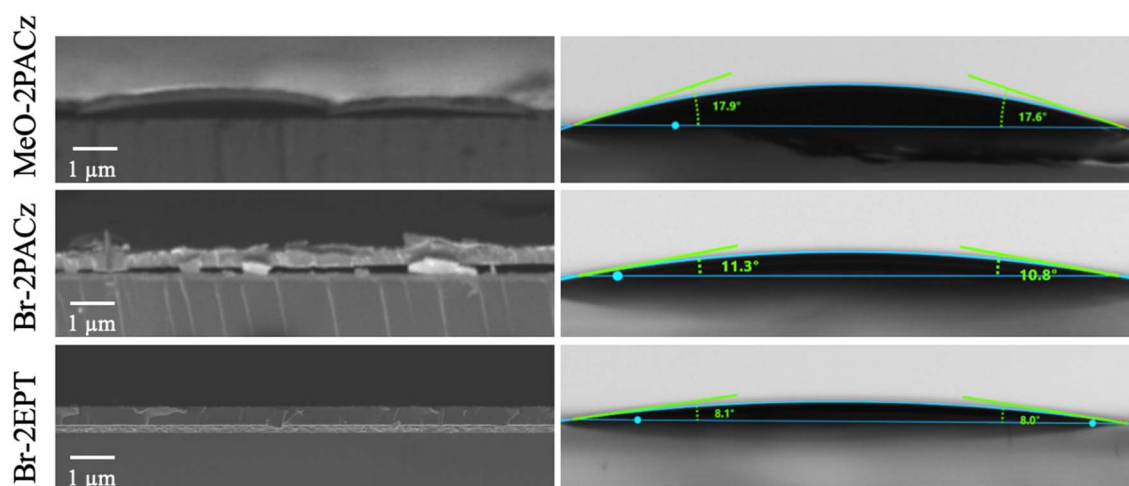
Fig. 2 Left: Cross-section SEM images of the PbS QD film on the modified ITO contact. Right: Contact angle measurements of the sessile drop (PbS:PbX2 ink in diluted butylamine) for different interlayers on ITO.
