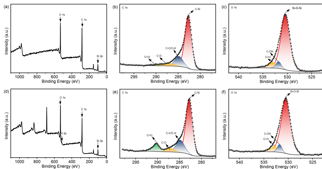
Fig. 4 XPS spectra of (a) acac(100)-PMO, in the regions of (b) C 1s and (c) O 1s; and (d) acac(100)-PMO@VO_acac, in the regions of (e) C 1s and (f) O 1s.
