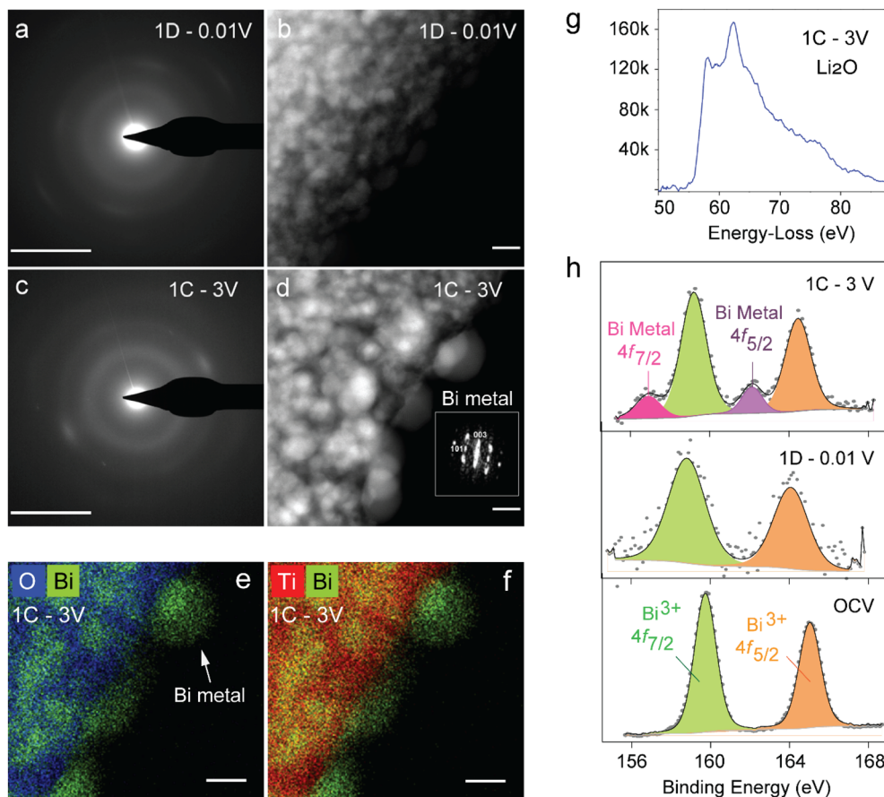
Fig. 5 Ex situ TEM and XPS analyses of NBT following lithium (de)insertion. SAED patterns and HAADF-STEM images of first discharged (a and b) and charged (c and d) samples. Bar size is equal to 5 nm -1 and 5 nm for the SAED patterns and HAADF-STEM images, respectively. (d) Fourier transformation of nanoparticles in the charged sample indexed to the R\bar{3}m structure of metallic Bi. (e and f) Color coded mixed EDS map of the charged sample, clearly showing the presence of bismuth metal and TiO 2 matrix that can be pictured as the plum-pudding model. (g) EELS spectrum of the foamy beam sensitive material (Fig. S2†) in the 1C sample near the Li K-edge region. (h) Bi 4f XPS spectra of pristine NBT (bottom) after first discharge (middle) and charge (top).
