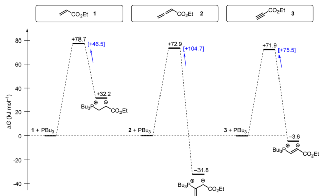
Fig. 18 Gibbs energy profiles for PBu 3 additions to Michael acceptors 1, 2 and 3 in dichloromethane solution. Experimentally determined Gibbs activation energies ΔG ‡ exp are combined with quantum-chemically calculated reaction energies ΔG add (data from Table 4). Reaction barriers for the retro-additions [ΔG ‡ retro ] are given in square brackets.
