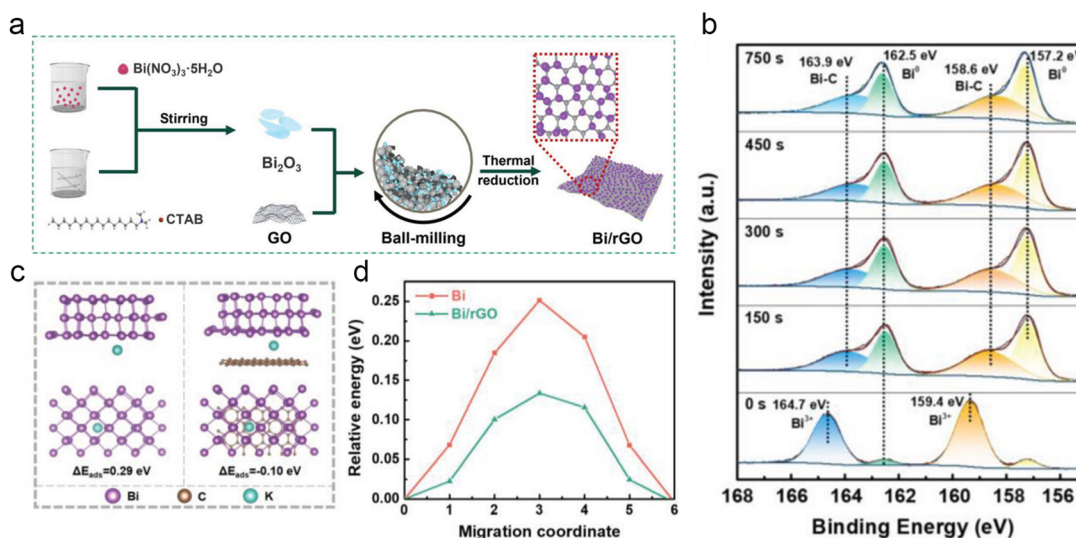
Fig. 7 (a) Schematic illustration for the preparation of Bi/rGO composites. (b) XPS Bi 4f spectra of Bi/rGO-2. (c) Potassium adsorption on the surface of Bi (112) and the interface of Bi/rGO. (d) The K^+ diffusion barrier energy in the Bi and Bi/rGO. Reproduced with permission. 51 Copyright 2024, Wiley-VCH.
