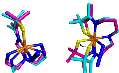
Fig. 12 Visualization of experimentally obtained structural changes that occur upon oxidation and binding of a sixth ligand, azide. Left: [Fe II (S Me2 N 3 (tren))] (4, cyan) 36 to [Fe III (S Me2 N 3 (tren))N 3 ] (magenta). 37 Right: [Fe II (S 2 Me2 N 3 (Pr,Pr))] ( 1 , cyan) 22 and [Fe III (S 2 Me2 N 3 (Pr,Pr))(N 3 )] (magenta). 31 Depiction utilized previously reported crystallographically determined structures.
