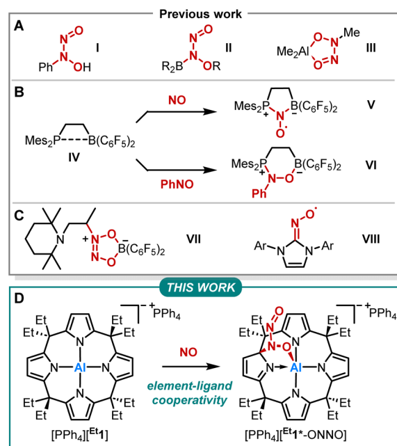
Fig. 1 (A–C) Previously reported reactivities of NO and nitrosobenzene with main-group element compounds. (D) Reactivity of calix[4]pyrrolato aluminate ([Et1] − ) with NO studied within this work. The asterisk in [Et1*-ONNO] − indicates the dearomatization of one pyrrole unit.
