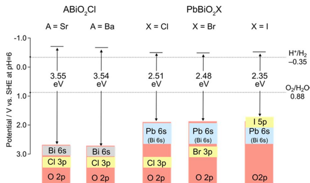
Fig. 5 Band alignments and band structures of Sillén-type \text{MBiO}_2\text{X} ( M = \text{Sr}, \text{Ba}, \text{Pb}; X = \text{Cl}, \text{Br}, \text{I} ). 33
