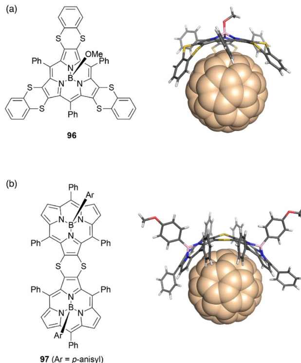
Fig. 10 Crystal structures of fullerene complexes (a) 96 · C_{60} and (b) 97 · C_{70} .
