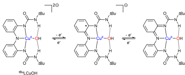
Scheme 9 Characterized oxidation states reached via reduction/oxidation of t Bu 2 LCuOH. Adapted from ref. 73.
