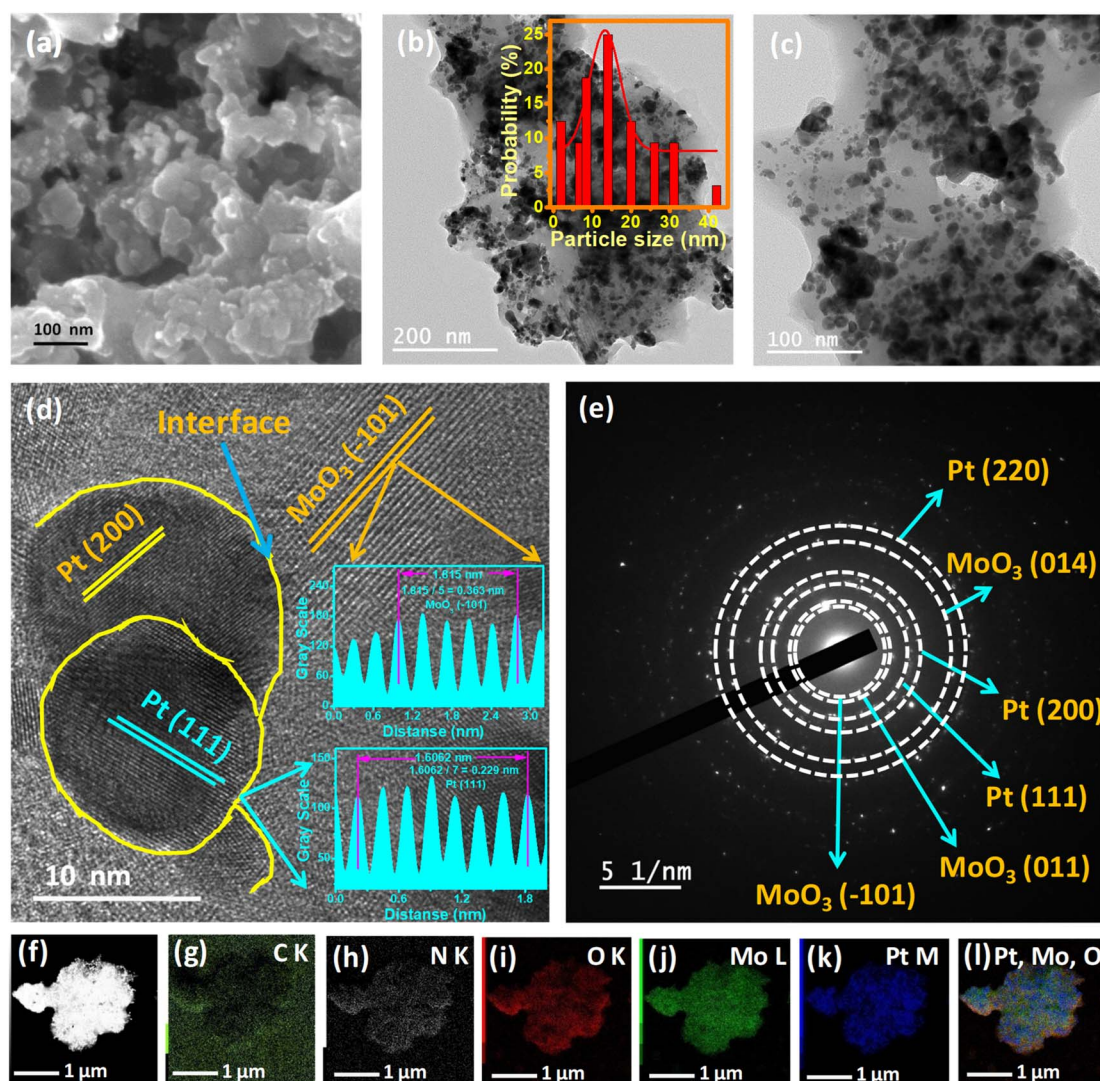
Fig. 1 (a) FE-SEM, (b and c) TEM, (d) HRTEM, and (e) SAED images of \text{Pt}/\text{MoO}_3\text{-CN}_x -400. (f–k) STEM and elemental mapping images of \text{Pt}/\text{MoO}_3\text{-CN}_x -400. (l) Elemental mapping overlay of Pt, Mo, and O.
