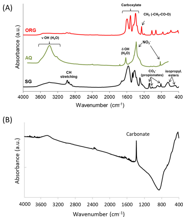
Fig. 2 FTIR spectra of (A) the AQ, ORG and SG precursors and (B) the SG sample calcined at 1200 ^\circ\text{C} .
