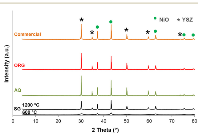
Fig. 3 X-ray diffraction patterns of SG (calcined at 600 and 1200 ^\circ\text{C} for 5 h) and AQ, ORG and the NiO–YSZ commercial samples calcined at 1200 ^\circ\text{C} for 5 h (JCPDF files: NiO: 01-089-5881; YSZ: 01-070-4431).
