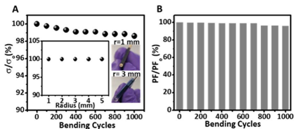
Fig. 4 (A) Relative electrical conductivity vs. bending cycles of a nano-rough PEDOT:Tos/PDAC/PET film with a specific bending radius of 1 mm. Inset: the relative electrical conductivity of the nano-rough PEDOT:Tos/PDAC/PET as a function of bending radius for one bending cycle and photos showing bending of the nano-rough PEDOT:Tos/PDAC/PET films across a cylindrical rod with radius of 1 mm and 3 mm, and (B) relative power factor of the film before and after bending as a function of bending cycle with a bending radius of 1 mm.
