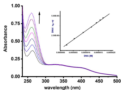
Fig. 2 Electronic absorption spectrum of complex Ru2 in the presence of increasing concentration of CT-DNA in PBS buffer. (Inset) Plot of [CT-DNA]/(\epsilon_a - \epsilon_f) vs. [DNA] . The arrow depicts hyperchromic shift on the addition of increasing quantities of DNA.
