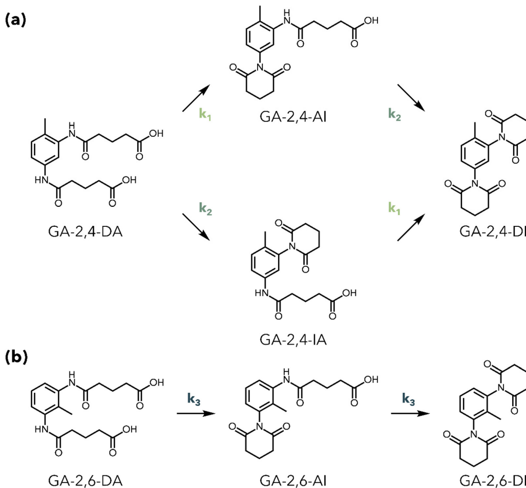
Scheme 2 Proposed kinetic model for amide/imide formation during M-PUF acidolysis with GA. (a) Shows the reaction pathways of 2,4-isomers, while (b) shows the reaction pathway of 2,6-isomers. Here we assume that the rate constant for the formation of an imide is dependent on its location relative to the other groups on the ring but not the chemical identity of the other (non-reacting) N-containing group on the ring ( i.e. , whether it is an amide or an imide), resulting in a reduced model with three rate constants that can all be estimated with reasonable confidence intervals.
