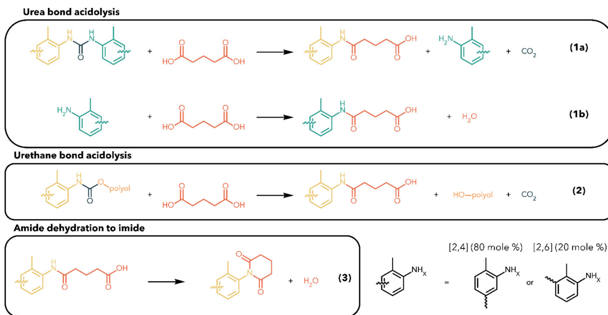
Scheme 1 Reaction stoichiometry of acidolysis of a flexible PUF with GA. (1a) Reaction of a urea bond to produce an amide, amine, and \text{CO}_2 ; (1b) reaction of amine intermediate with excess GA to produce an amide and \text{H}_2\text{O} ; (2) reaction of a urethane bond to produce an amide, polyol, and \text{CO}_2 ; (3) reaction of an amide product to produce an imide and \text{H}_2\text{O} . Legend: aromatic groups in most flexible PUFs are derived from TDI, which is synthesized as an isomeric mixture of 2,4-TDI (80 mol%) and 2,6-TDI (20 mol%).
