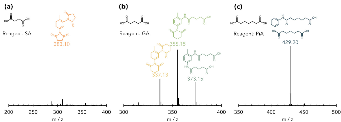
Fig. 3 UPLC-MS spectra of reaction products from M-PUF acidolysis with (a) SA, (b) GA, and (c) PiA. Reaction conditions: 0.5 g M-PUF, 1.5 g DCA, 195 °C, 2 hours under an N 2 atmosphere. After 2 hours, the reactions were quenched in ice, and a ca. 1 mg sample was extracted and dissolved in methanol for UPLC-MS analysis.
