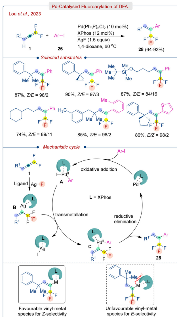
Scheme 14 Pd-Catalyzed fluoroarylation of DFA.
