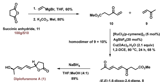
Scheme 2 Highly concise synthesis of diplofuranone A (1).
