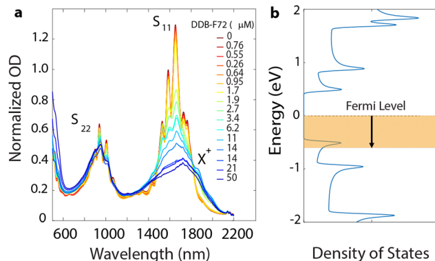
Fig. 1 (a) Absorption spectra of DDB-F72 doped s-SWCNT. Undoped sample (dark red, 0 \mu\text{M} DDB-F72) transitions to the highly doped sample (dark blue, 50 \mu\text{M} DDB-F72). Color code guide corresponds to dopant concentration for each trace. (b) Fermi energy shift because of molecular doping, modelling the phase-space filling effect. Calculated density of states (DOS) corresponds to (10,8) chirality.
