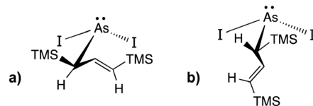
Fig. 3 (a) Preferred conformation of an [AsA'I_2] unit when the [AsI_2] fragment is part of the AsI_3 lattice; (b) Lowest energy conformation of an [AsA'I_2] unit in solution. TMS = trimethylsilyl.
