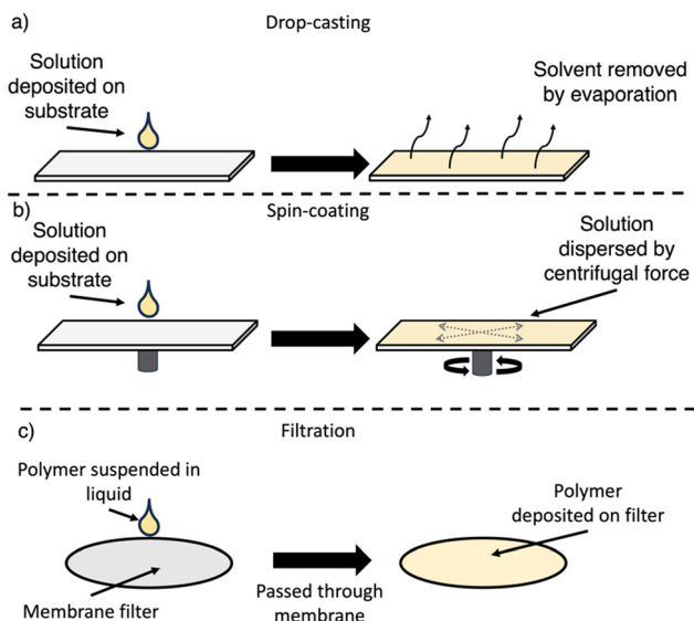
Fig. 21 Outlines of procedures used to fabricate film photocatalysts. (a) drop-casting method; (b) spin-coating method (N.B. spin-coating can be performed with substrate static or while spinning.); and (c) filtration.
